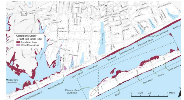
Figure 22: 1-Foot of Sea Level Rise
