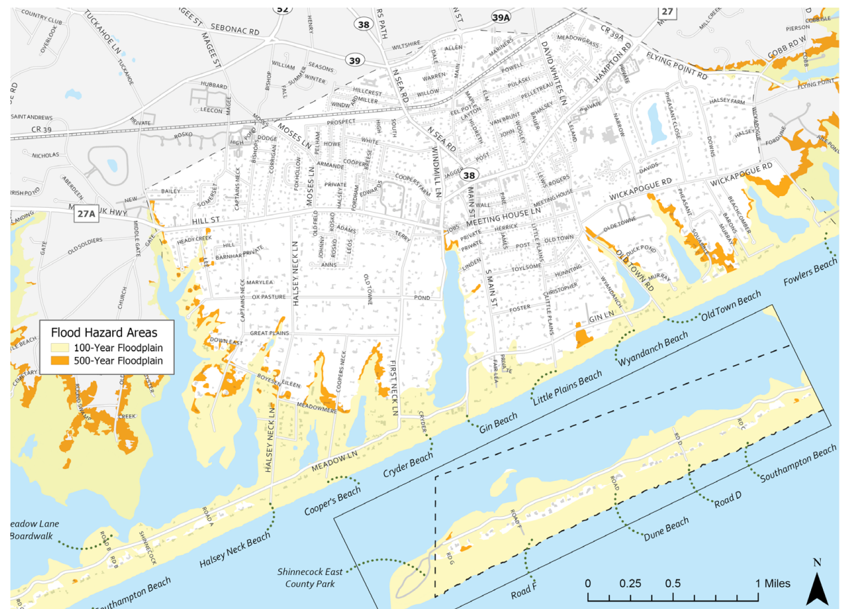
Figure 20: Flood Hazard Areas
